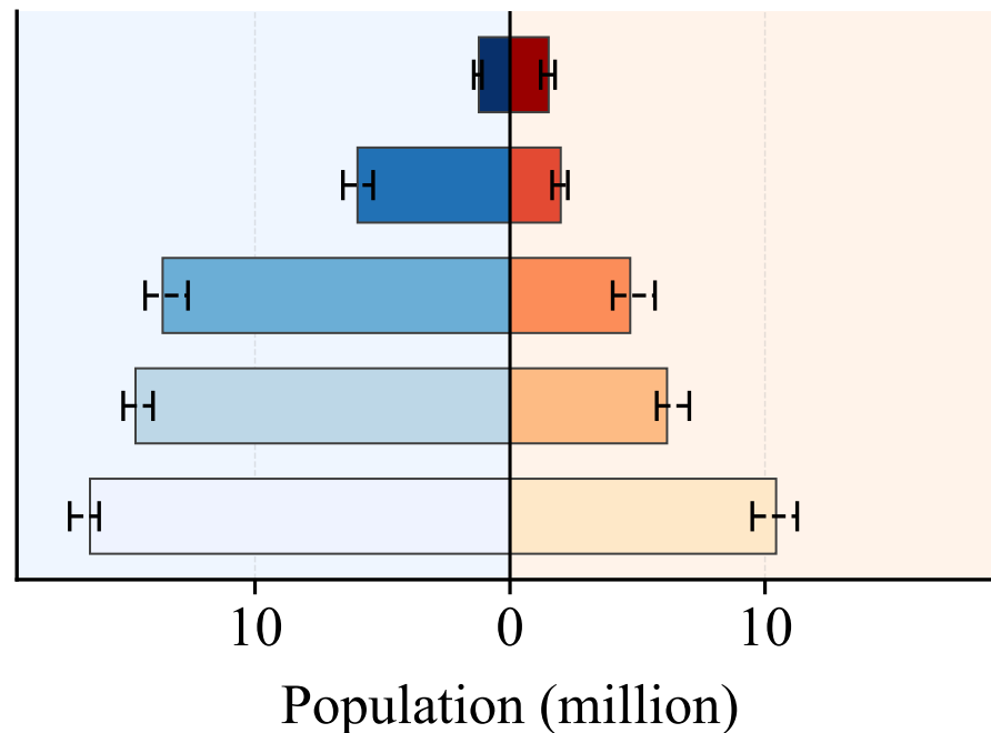
(b) CorrDiff - CMAQ (36 km)
